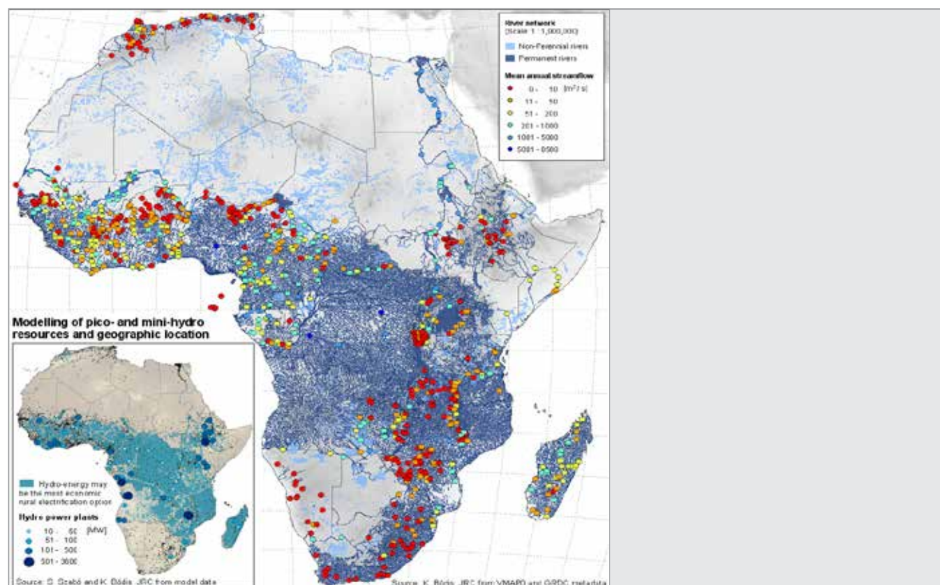
Figure 5.10: Hydro Resources and Locations of Hydro Plants in Africa
