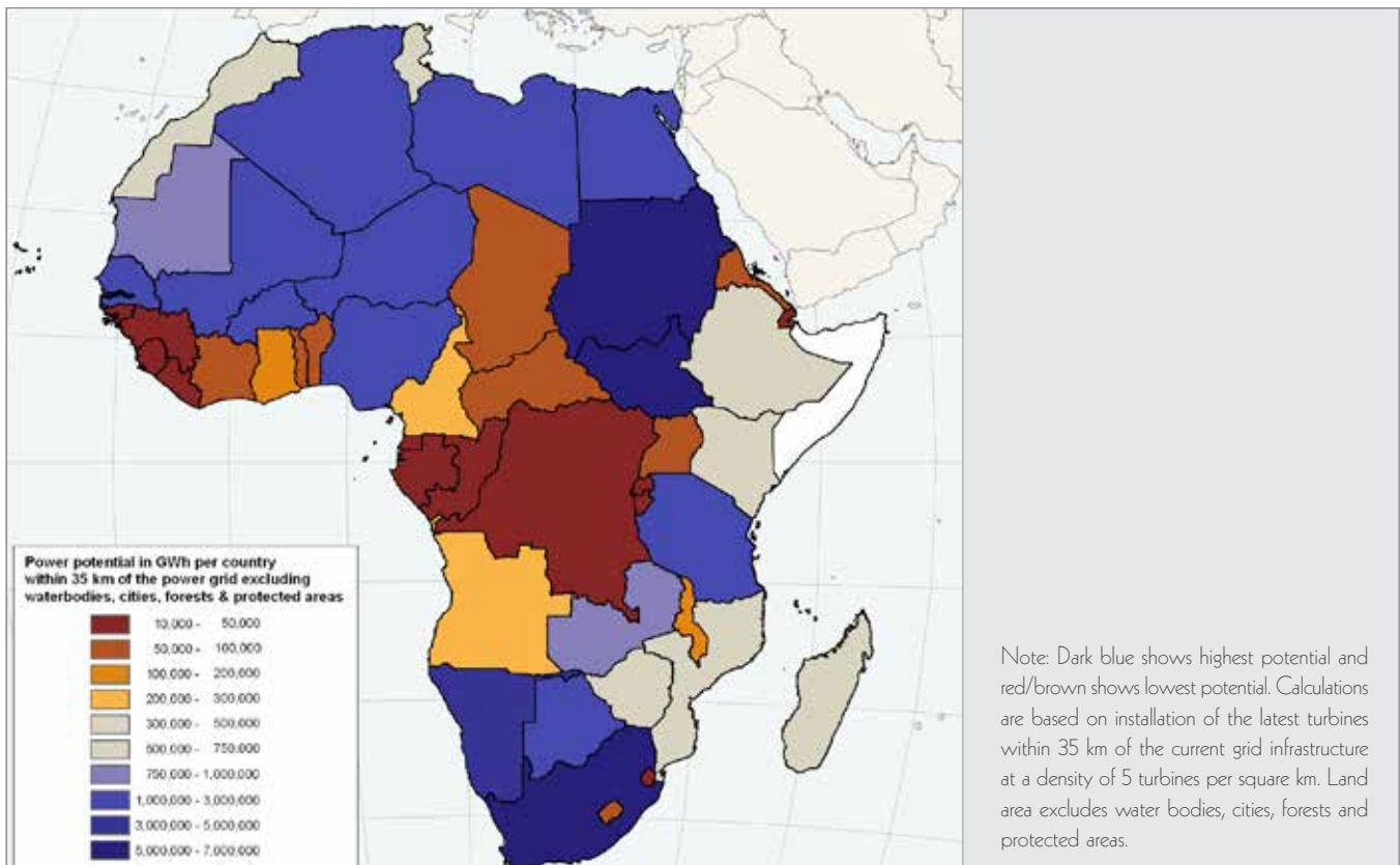
Figure 5.5: Power Potential of Onshore Wind Energy Resources per Country
